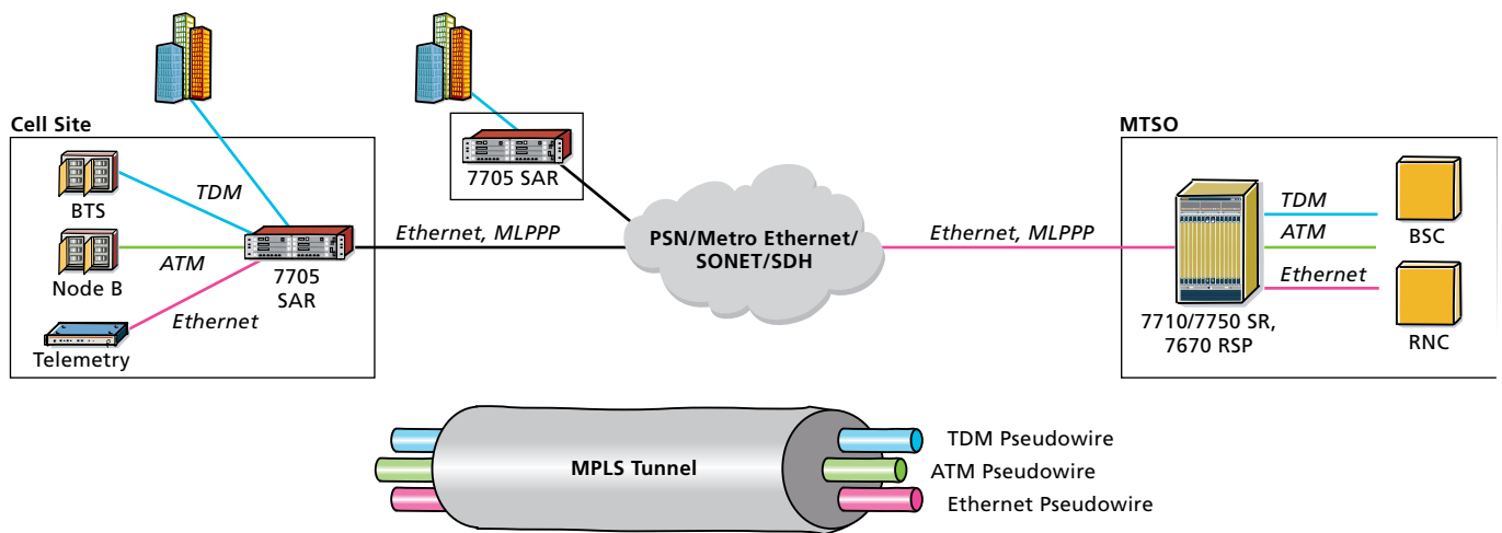
Figure 1. IP/MPLS RAN Transport Capability
