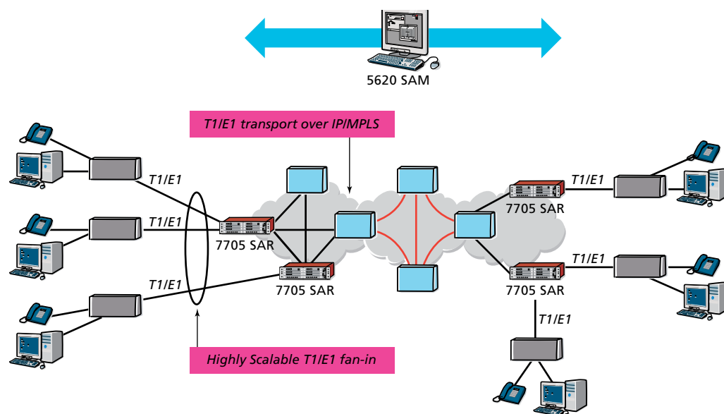
Figure 2. T1/E1 Private Line Transport Capability
